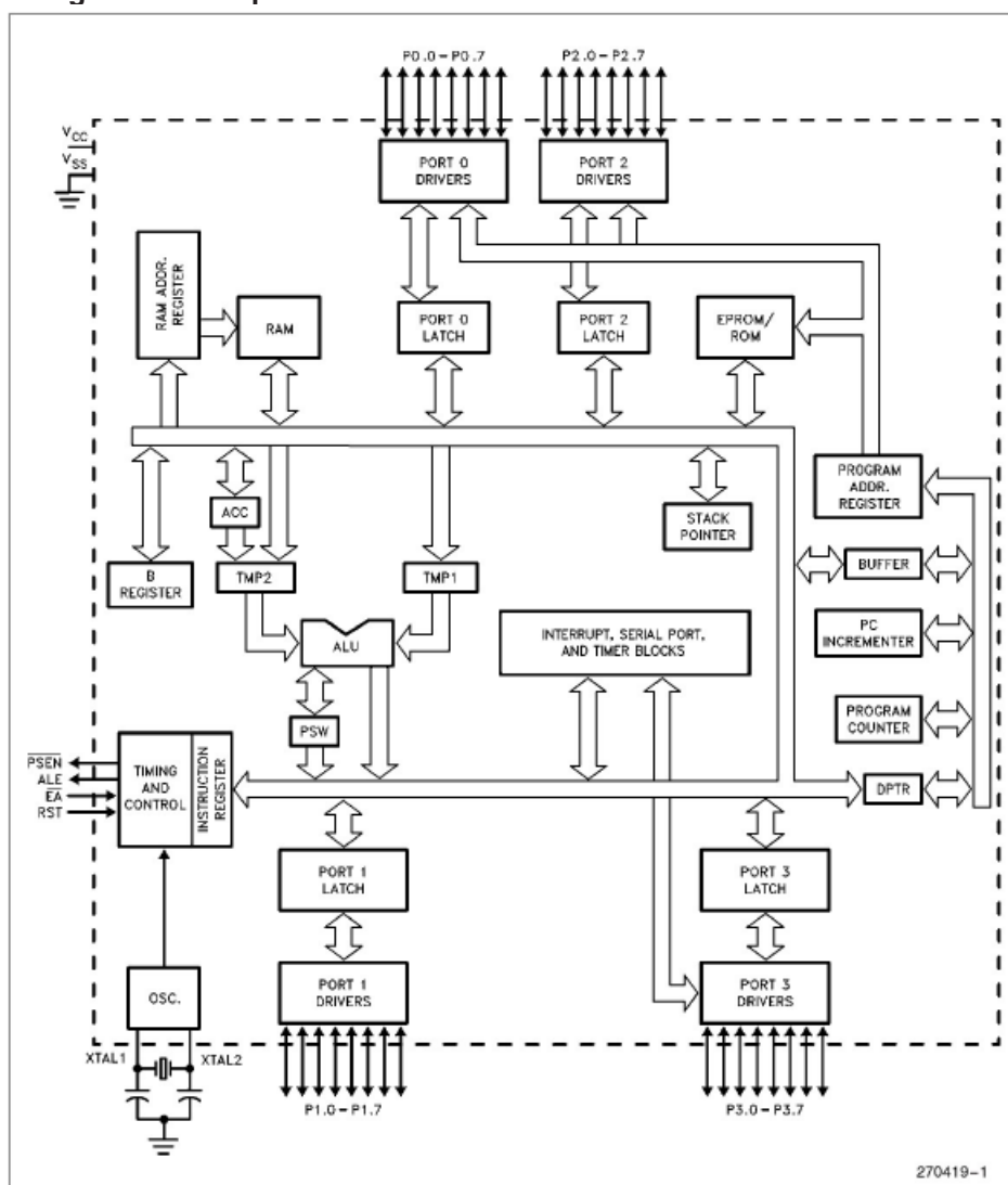
Figure 1. MCS® 51 Microcontroller Architectural Block Diagram
